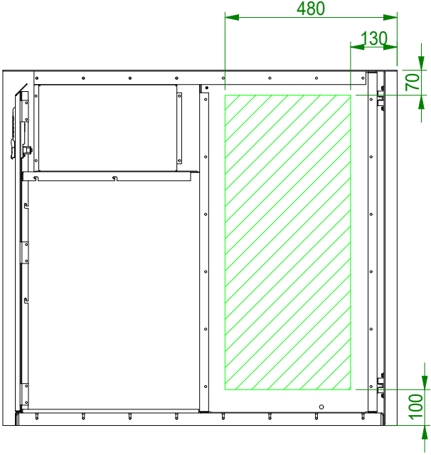
OPTION LED LOGO max dimensions for lasercutting logo
