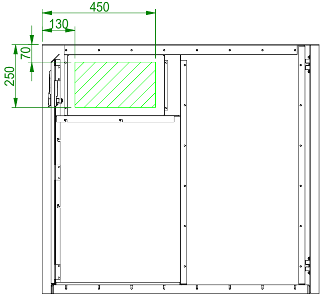
OPTION LED NUMBER max dimensions for lasercutting number
